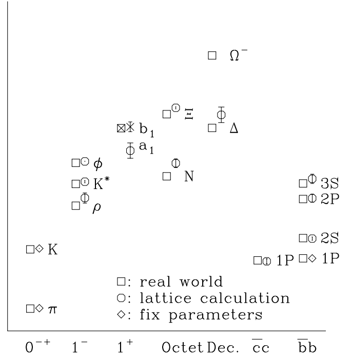
FIG. 17. The “big picture.” Crude continuum and chiral extrapolations of hadron masses and splittings compared with experimental values. The upson and charmonium columns are differences from the ground state masses, from work of the HPQCD and Fermilab groups [16,19]. Here the \pi and K masses fix the light and strange quark masses, and the Y 1P-1S mass splitting is used to fix the lattice spacing.
